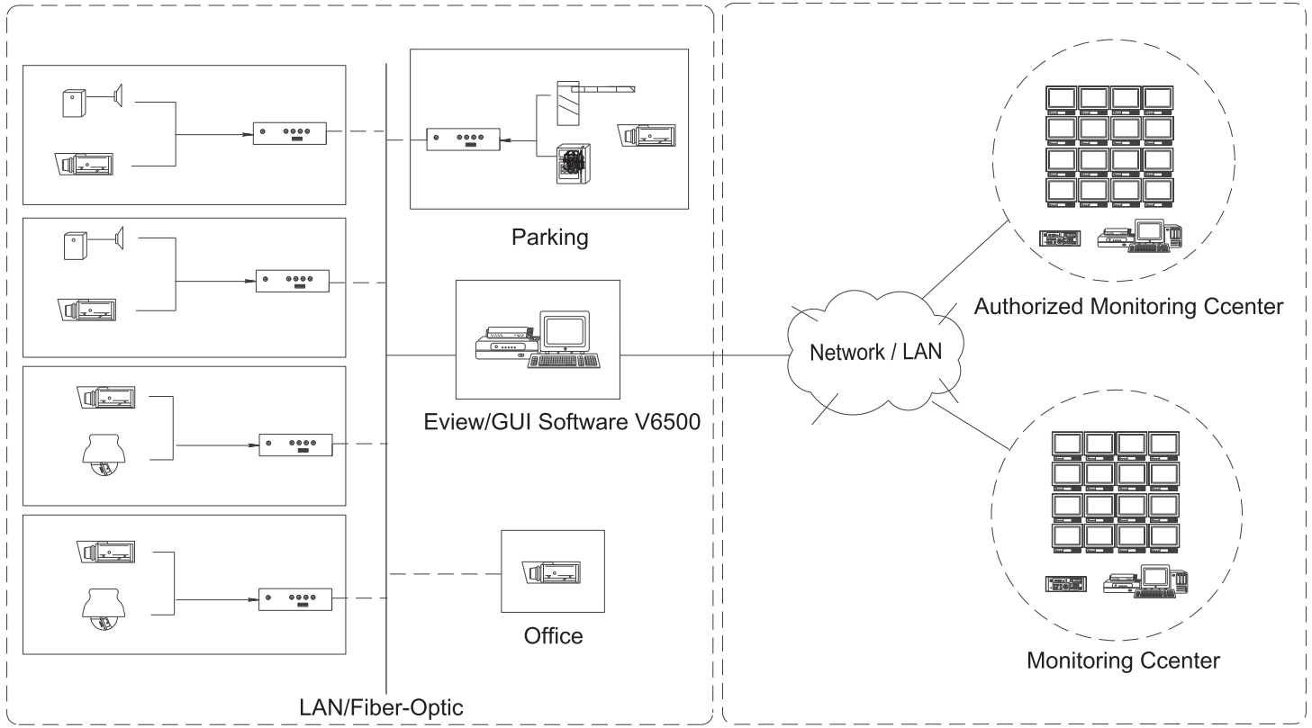
Network Monitoring Conformity System
